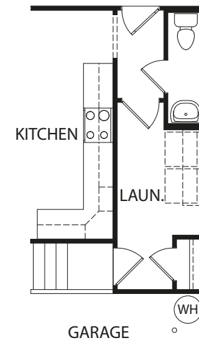
Main Level with Optional Second Level Loft
