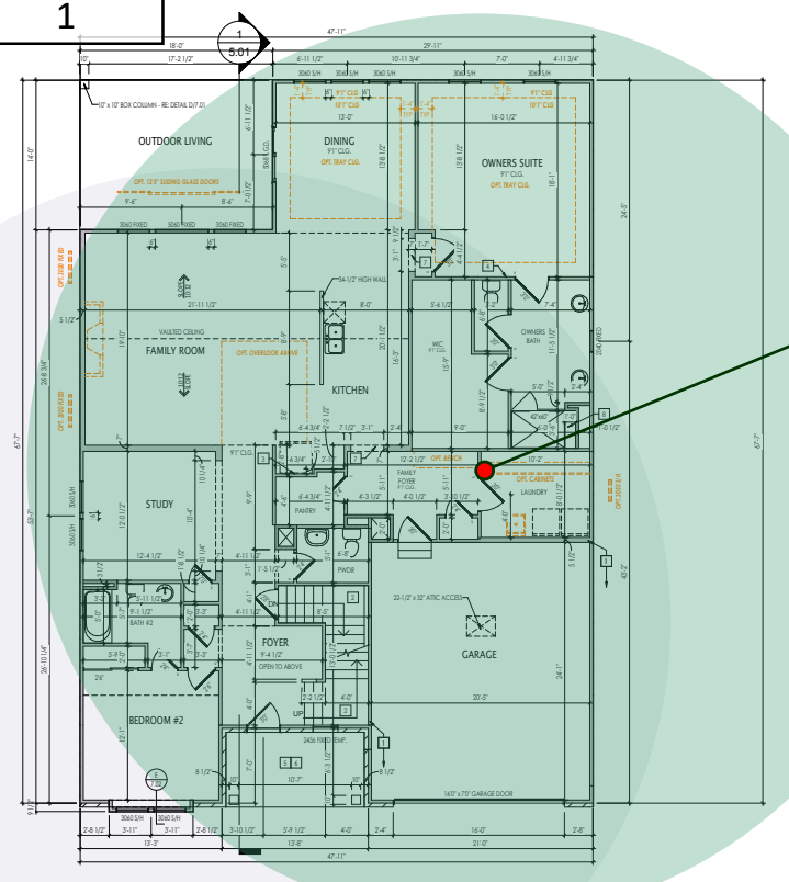
Wi-Fi coverage from the Wireless AP in the Second Floor Plan
