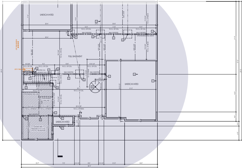
Wi-Fi coverage from the Wireless AP in the First Floor Plan
