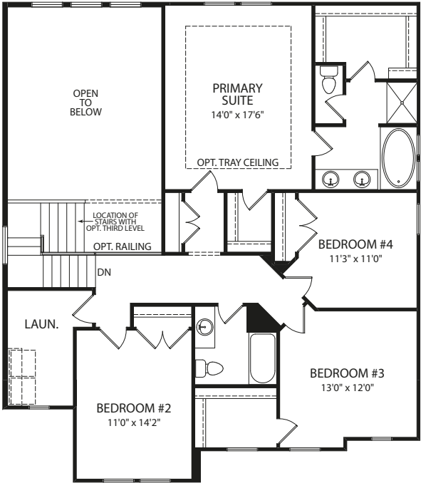
Second Level
