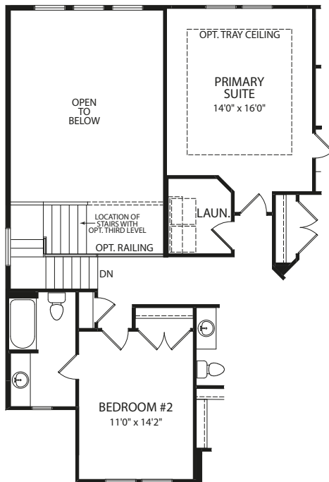
Optional Full Bath at Bedroom #2
