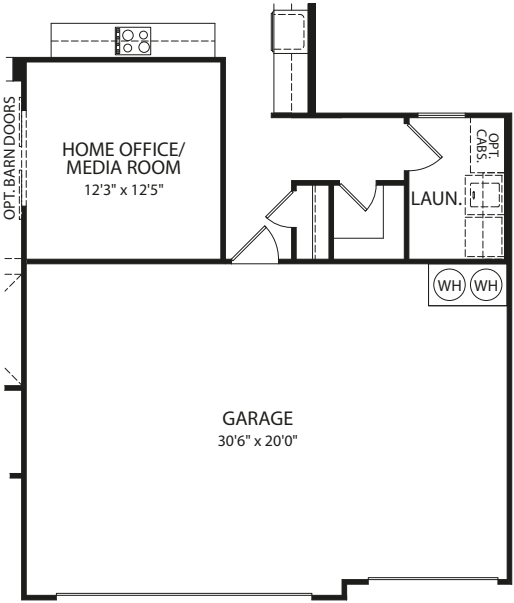
Optional 3-Car Front-Entry and Alternate Home Office/ Media Location
